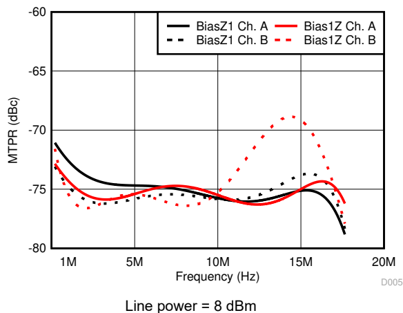
Figure 6-5. MTPR VDSL-17a Mode
