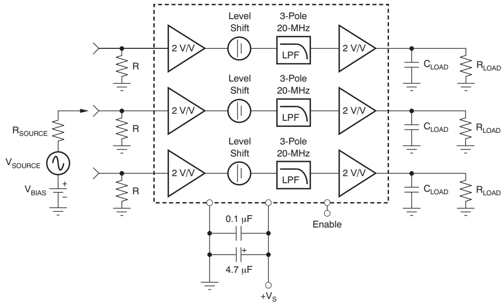
Figure 1. Test Circuit
