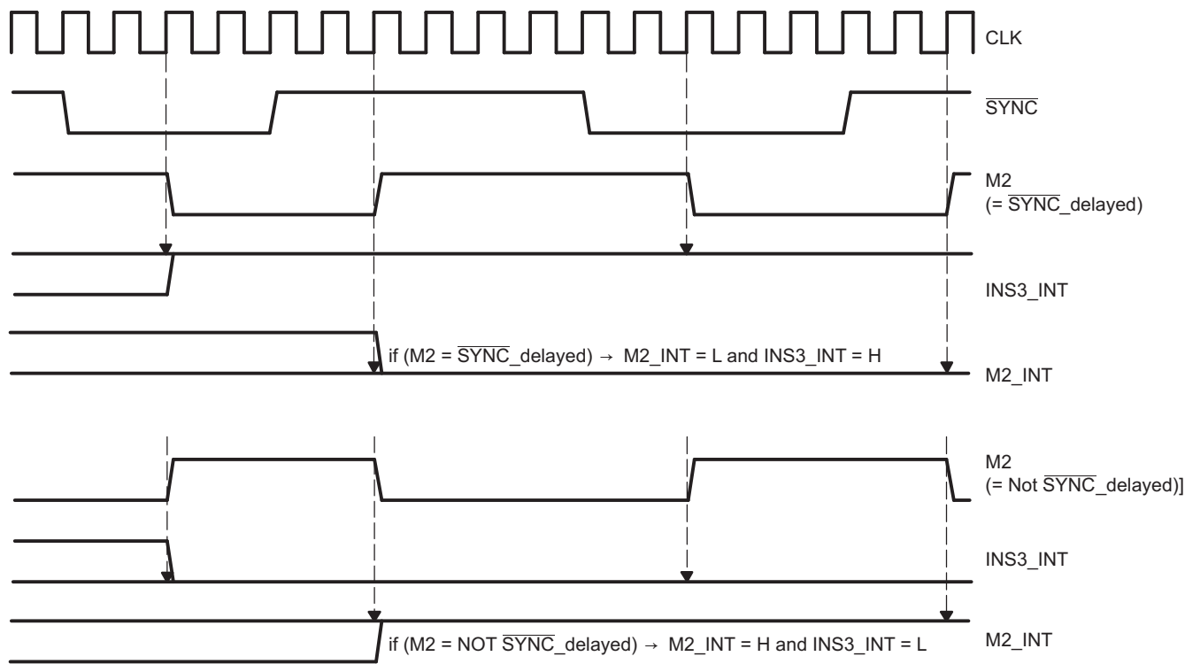
Figure 6. Generating INS3_INT and M2_INT From M2
