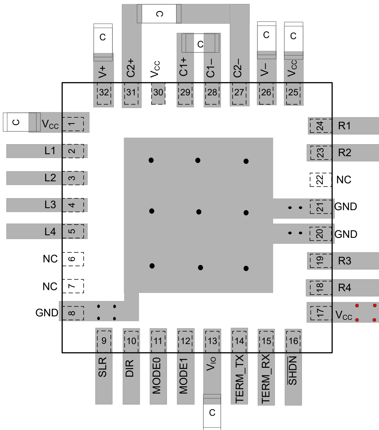
Figure 8-13. Layout Example
