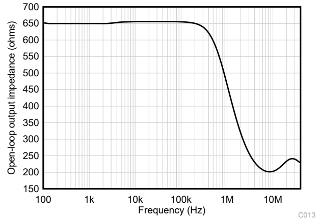
Figure 4-6. Output Loop Output Impedance vs Frequency
