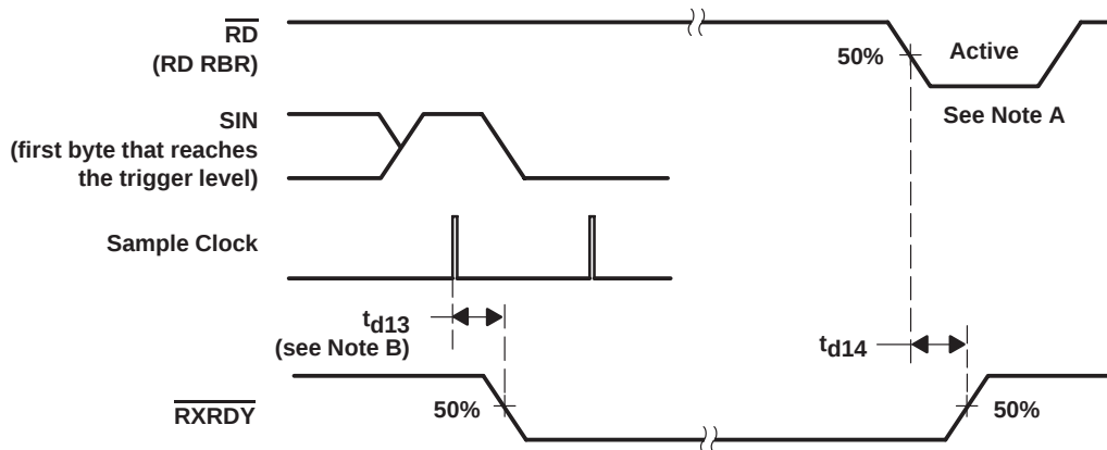
Figure 10. Receiver Ready (RXRDY) Waveforms, FCR0 = 0 or FCR0 = 1 and FCR3 = 0 (Mode 0)
