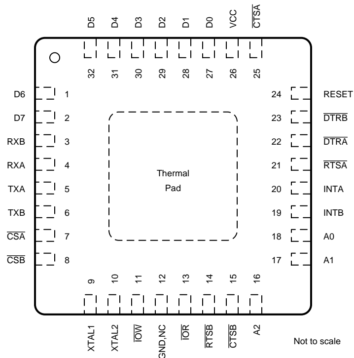
RHB Package 32-Pin VQFN Top View
