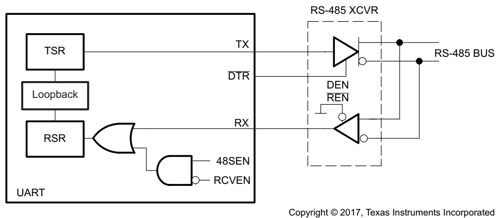
Figure 29. RS-485 Application Example 2
