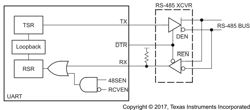
Figure 28. RS-485 Application Example 1
