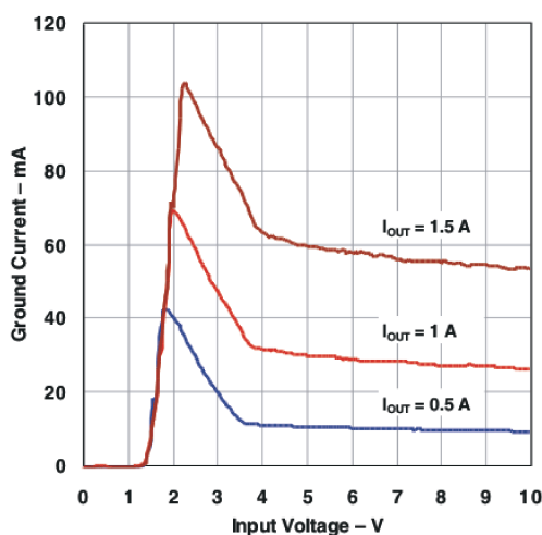
Figure 5-17. TL1963A-33 Ground Current vs Input Voltage (Legacy Chip)
