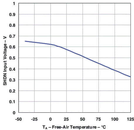
Figure 5-25. \overline{\text{SHDN}} Threshold (ON to OFF) vs Temperature (Legacy Chip)
