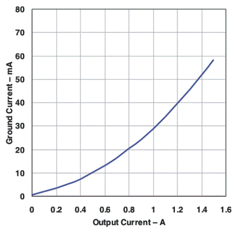
Figure 5-20. Ground Current vs Output Current (Legacy Chip)
