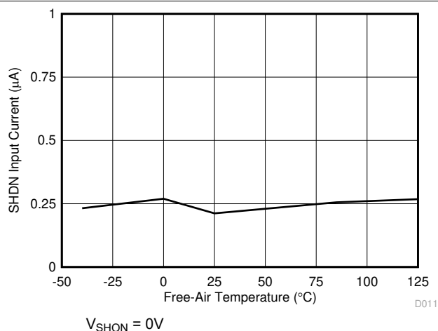
Figure 5-22. SHDN Pin Current ( I_{SHDN} ) vs Temperature (Legacy Chip)
