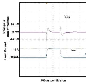
Figure 5-41. Load Transient Response (Legacy Chip)
