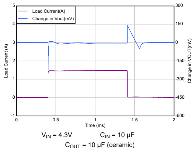
Figure 7-8. Load Transient Response (New Chip)
