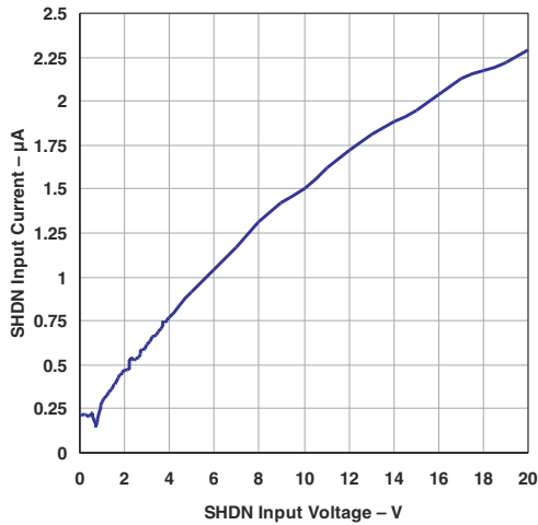
Figure 5-23. \overline{\text{SHDN}} Pin Current ( I_{\text{SHDN}} ) vs \overline{\text{SHDN}} Input Voltage (Legacy Chip)
