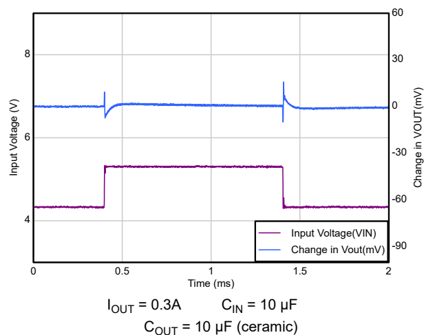
Figure 7-10. Line Transient Response (Legacy Chip)
