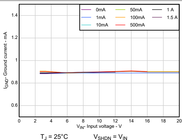
Figure 5-18. TL1963A-33 Ground Current vs Input Voltage (New Chip)
