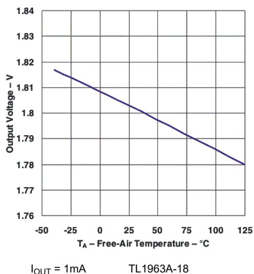
Figure 5-7. TL1963A-18 Output Voltage vs Temperature (Legacy Chip)
