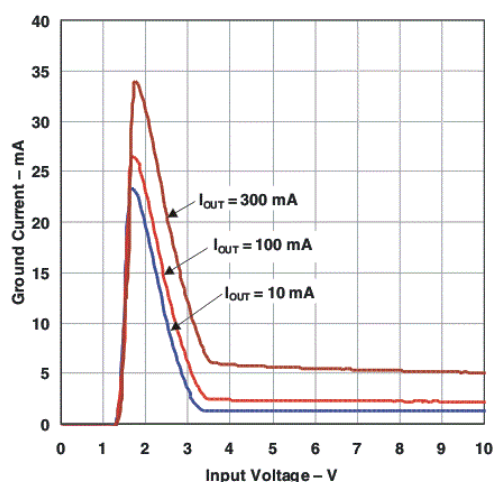
Figure 5-16. TL1963A-33 Ground Current vs Input Voltage (Legacy Chip)
