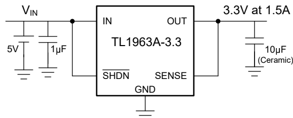
Figure 7-2. 4.3V to 3.3V Regulator
