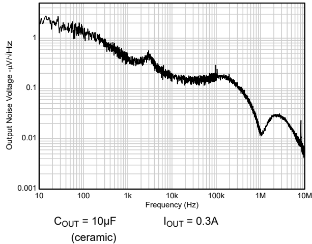
Figure 5-39. Output Noise Voltage vs Frequency (New chip)
