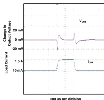
Figure 7-5. Load Transient Response (Legacy Chip)
