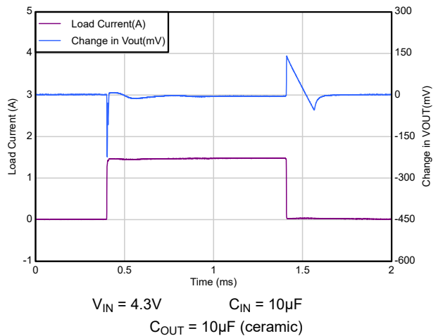
Figure 5-44. Load Transient Response (New Chip)
