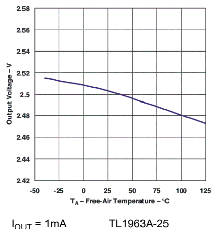
Figure 5-8. TL1963A-25 Output Voltage vs Temperature (Legacy Chip)
