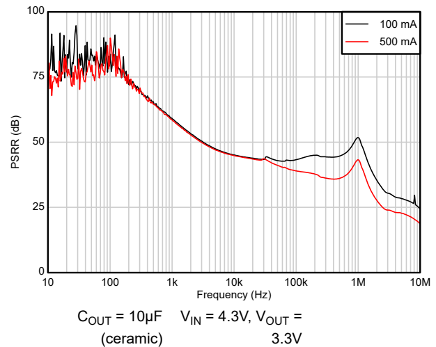
Figure 5-34. Ripple Rejection vs Frequency (New chip)
