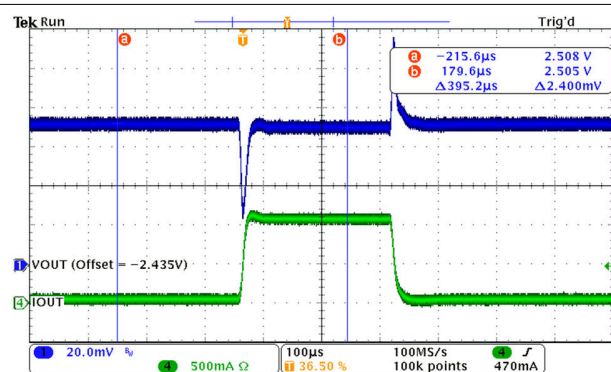
Figure 7-4. 1A Load Transient Response ( C_{OUT} = 10\mu F ) (Legacy chip)
