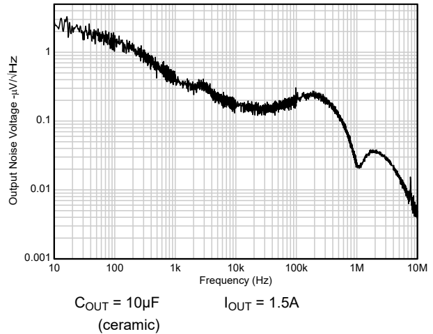
Figure 5-40. Output Noise Voltage vs Frequency (New chip)
