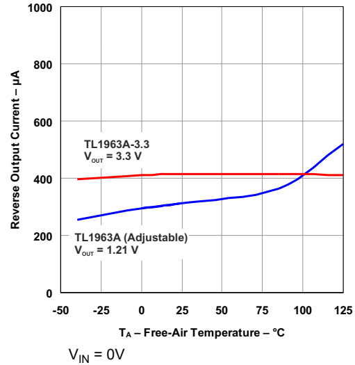
Figure 5-32. Reverse Output Current vs Temperature (Legacy Chip)
