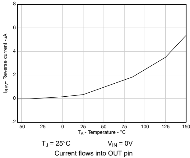
Figure 5-31. Reverse Output Current vs Temperature (New Chip)
