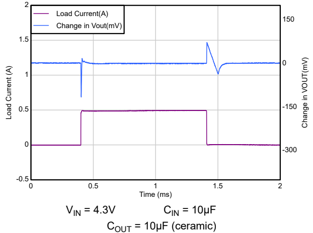
Figure 5-42. Load Transient Response (New Chip)
