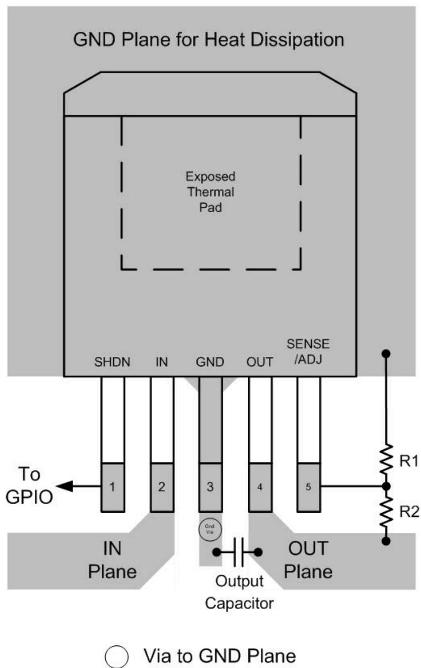
Figure 7-14. TO-263 Layout Example (KTT)
