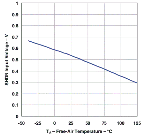
Figure 5-24. \overline{\text{SHDN}} Threshold (OFF to ON) vs Temperature (Legacy Chip)
