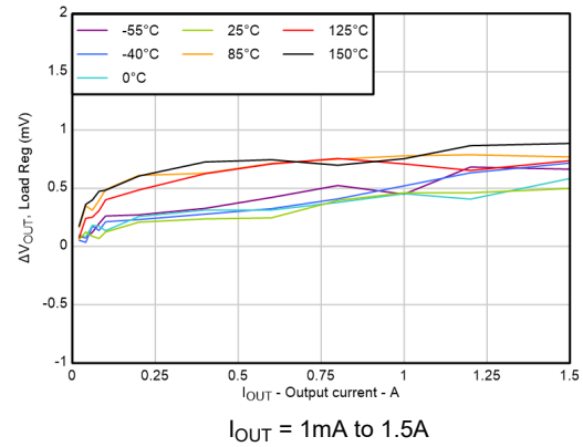
Figure 5-36. Load Regulation vs Temperature (New Chip)
