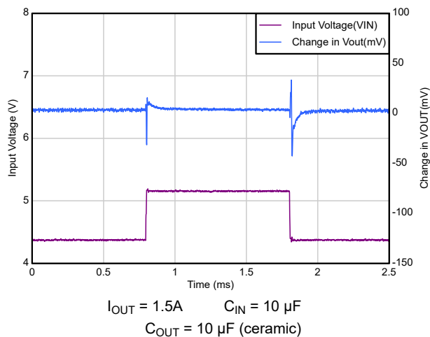
Figure 7-11. Line Transient Response (Legacy Chip)
