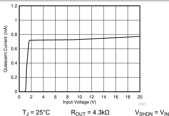
Figure 5-12. Quiescent Current vs Input Voltage (Legacy Chip)
