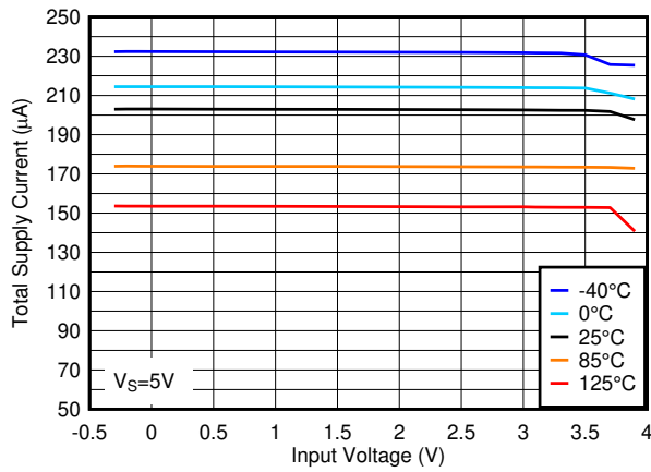
Figure 5-3. Total Supply Current vs. Input Voltage at 3.3V
