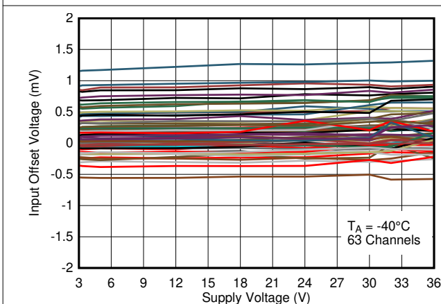
Figure 5-11. Input Offset Voltage vs. Supply Voltage at -40°C
