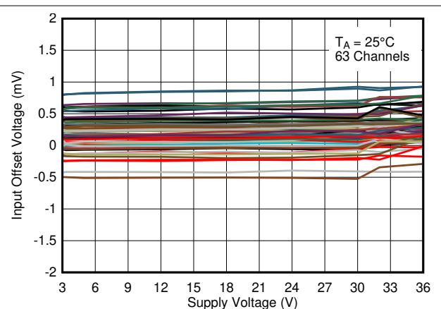
Figure 5-12. Input Offset Voltage vs. Supply Voltage at 25°C
