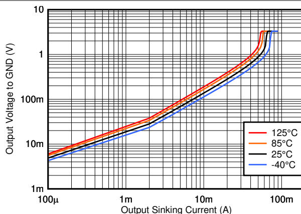
Figure 5-8. Output Sinking Current vs. Output Voltage, 3.3V
