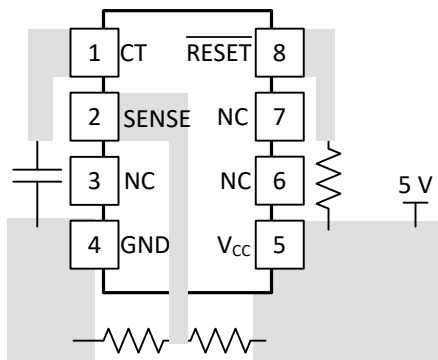
Figure 11-1. TL7700-SEP Layout
