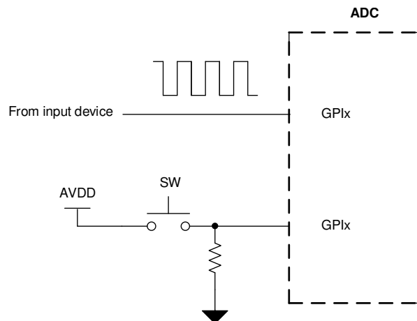
Figure 47. Digital Input
