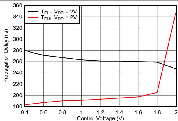
Figure 5-7. Propagation Delay vs Control Voltage
