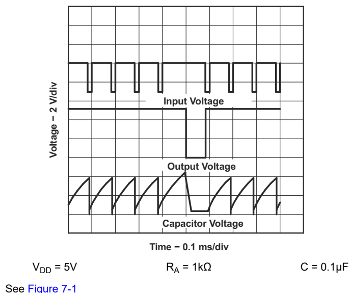
Figure 7-2. Timing Waveforms for Missing-Pulse Detector
