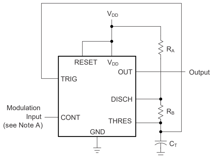
Figure 7-3. Circuit for Pulse-Position Modulation
