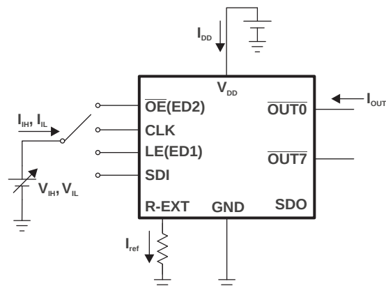
Figure 5. Test Circuit for Electrical Characteristics
