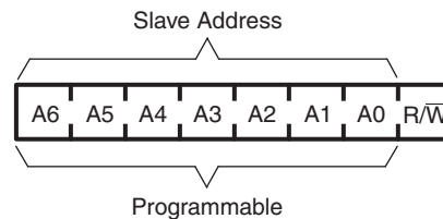
Figure 17. Slave Address
