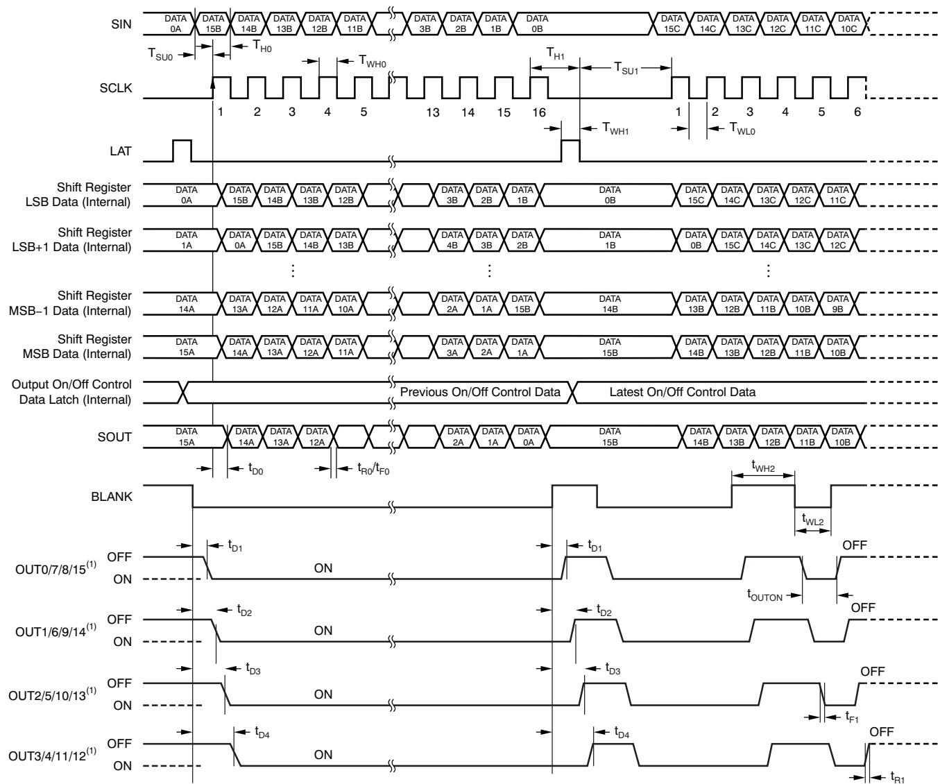
Figure 9. Timing Diagram
