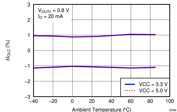
Figure 5-9. \Delta I_{OLC} vs Ambient Temperature
