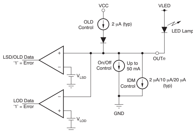
Figure 29. LOD/LSD/OLD/IDM Circuit
