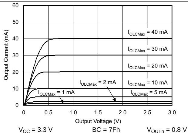
Figure 15. OUTn Current vs Output Voltage
