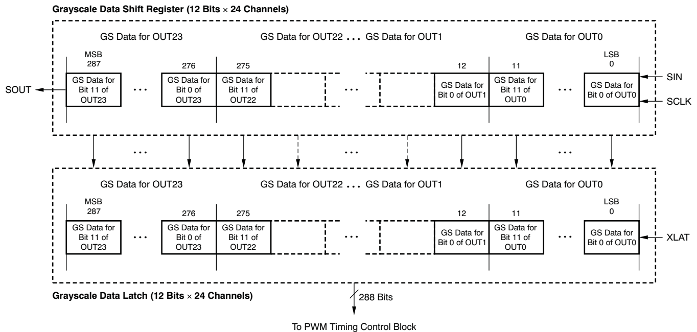
Figure 21. Grayscale Data Shift Register and Latch Configuration
