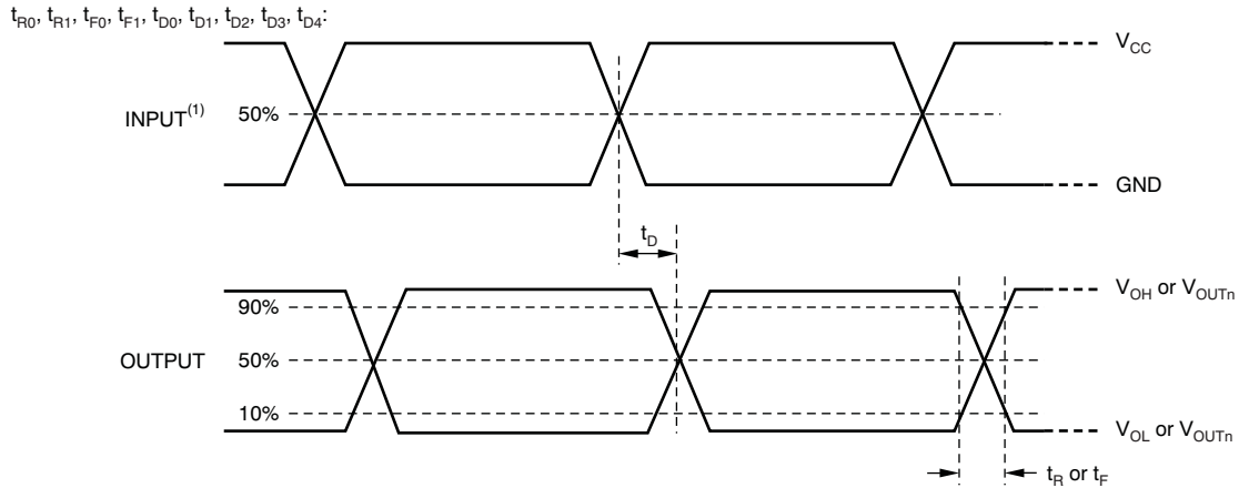
Figure 2. Output Timing
