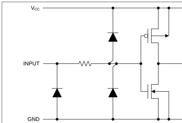
Figure 12. SIN, SCLK
