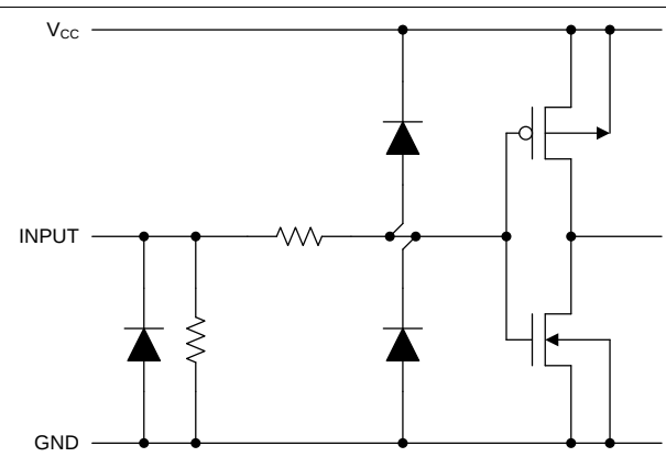
Figure 13. LAT, GCLK
