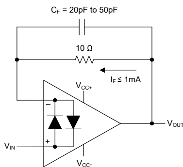
Figure 7-1. Voltage Follower
