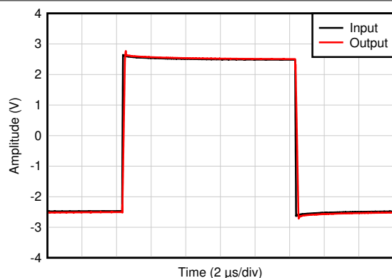
Figure 6-13. Small-Signal Pulse Response
