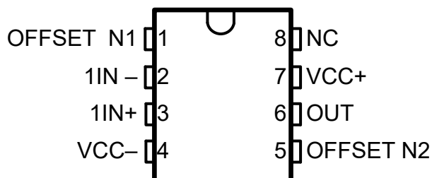
Figure 5-2. TLE2071 and TLE2071A JG PACKAGE (Top View)
