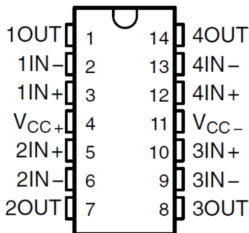
Figure 5-4. TLE2074 and TLE2074A J, N, OR W PACKAGE (Top View)
