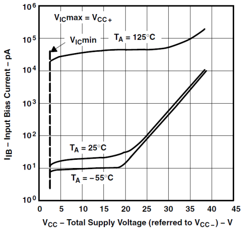
Figure 6-9. Input Bias Current vs Total Supply Voltage
