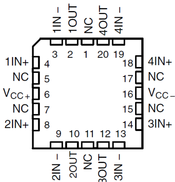
Figure 5-8. TLE2074M and TLE2074AM FK PACKAGE (Top View)
