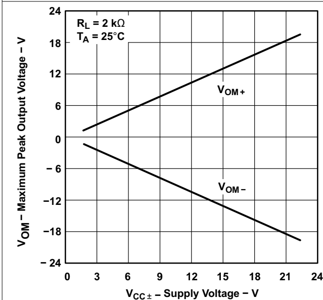
Figure 5-7. Maximum Peak Output Voltage vs Supply Voltage
