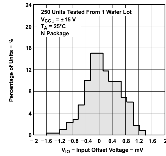
Figure 5-1. TLE2141 Distribution of Input Offset Voltage
