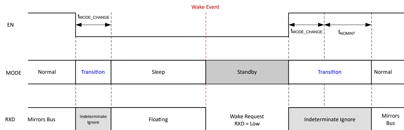
Figure 8-15. Mode Transitions
