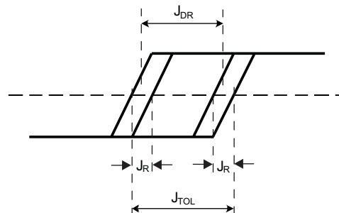
Figure 2. Pre/Post Cursor Swing Definitions
