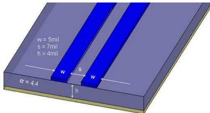
Figure 35. Differential Microstrip PCB Trace Geometry Example
