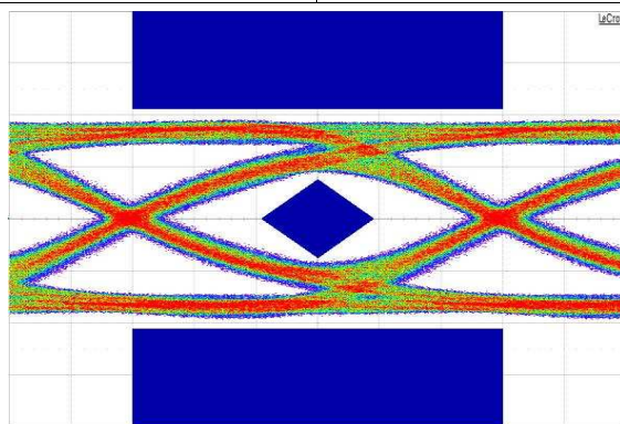
Figure 6. Transmitter Output (4-Inch FR-4 Trace)
