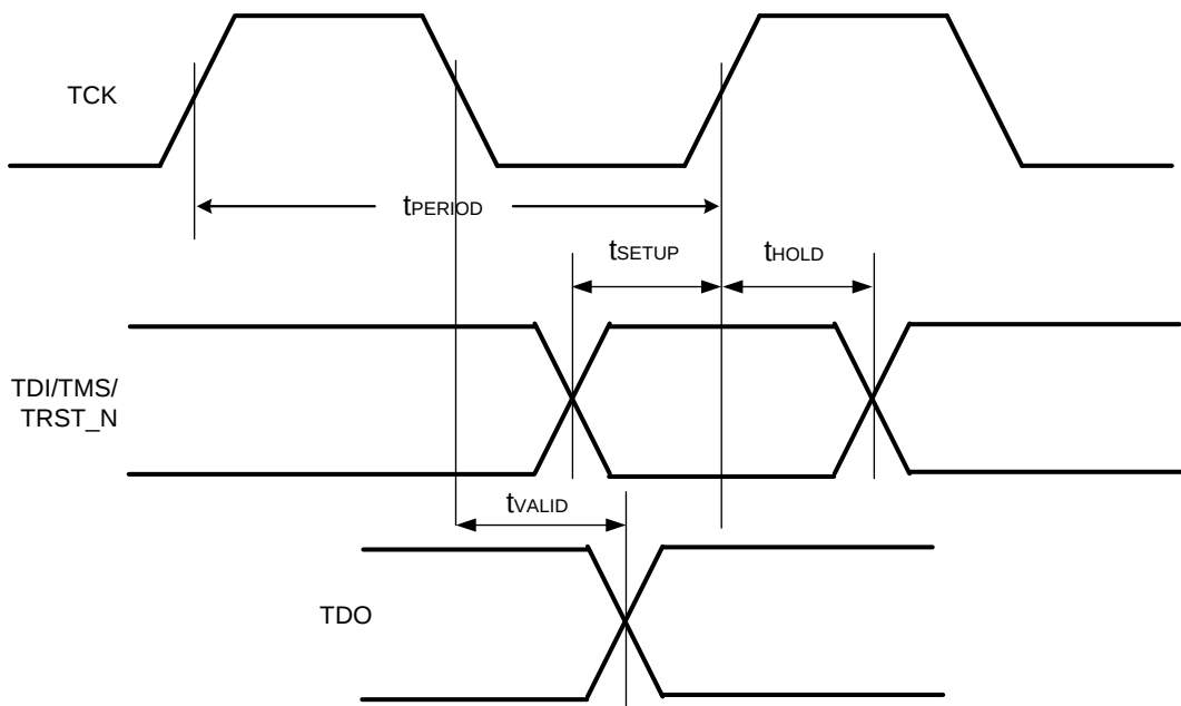
Figure 7-5. JTAG Timing
