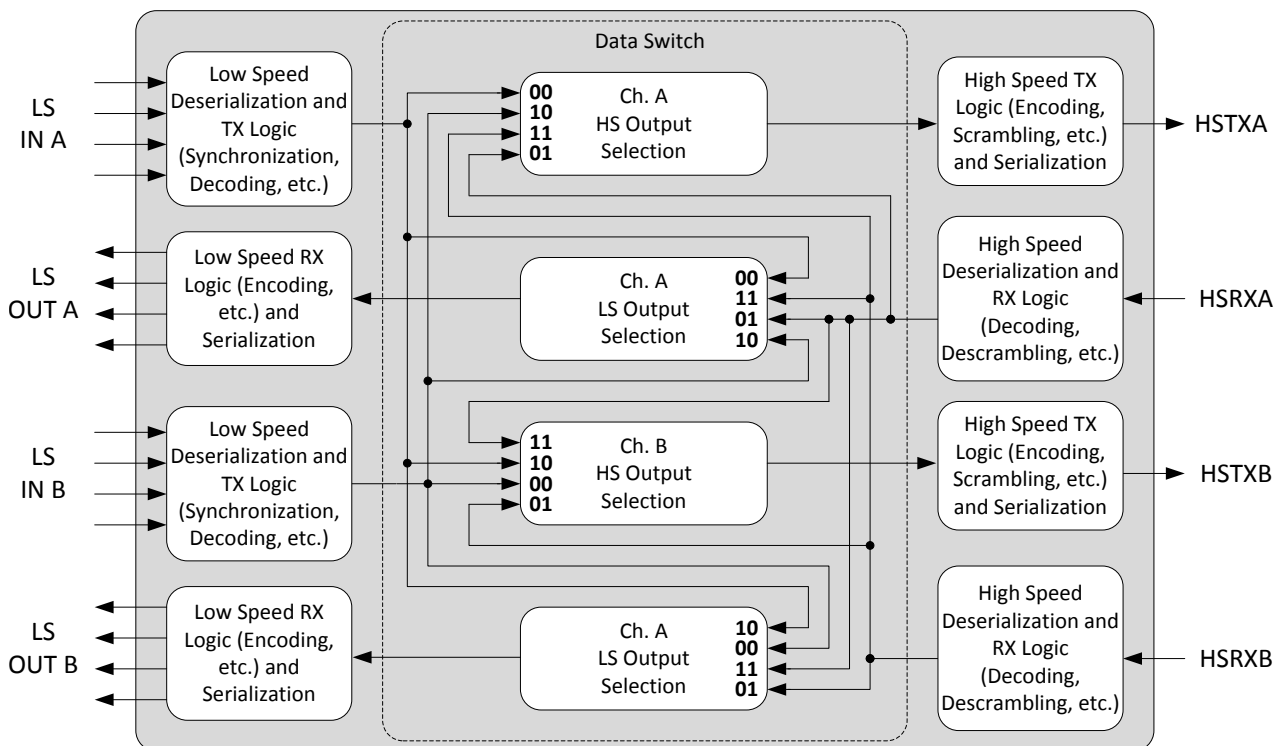
Figure 7-1. Signal Routings for Integrated Smart Switch
