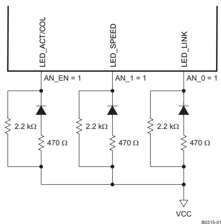
Figure 3-6. AN Pin Configuration and LED Loading Example
