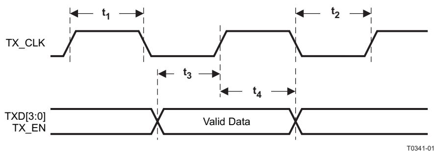
Figure 9-4. 100Mb/s MII Transmit Timing
