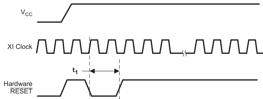
Figure 9-2. Reset Timing
