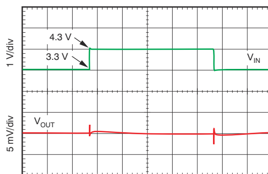
200 \mu\text{s}/\text{div} V_{OUT} = 1.8\text{ V} , I_{OUT} = 500\text{ mA}
