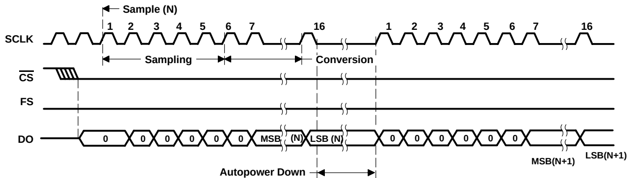
Figure 9. μC Application Timing Diagram
