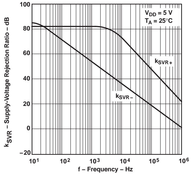
Figure 35. TLV2264
