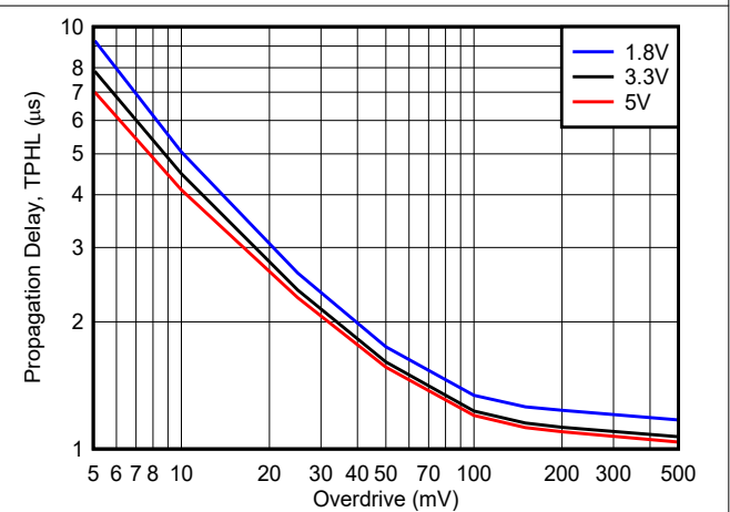
Figure 8-12. High to Low Propagation Delay vs. Overdrive
