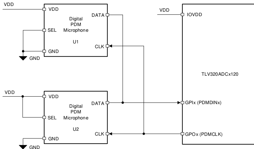
Figure 8-64. Digital PDM Microphones Connection Diagram for the TLV320ADC3120
