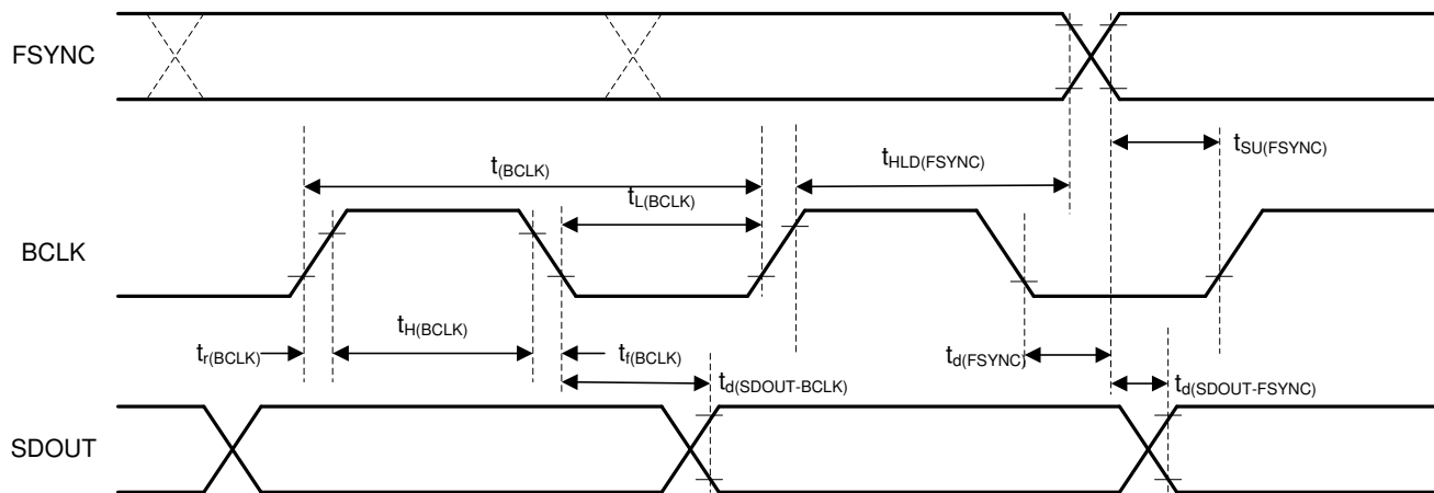
Figure 3. TDM (With BCLK_POL = 1), I 2 S, and LJ Interface Timing Diagram
