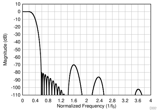
Figure 49. Linear Phase Decimation Filter Magnitude Response
