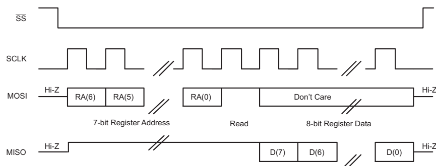
Figure 88. SPI Single-Byte Read Transfer
