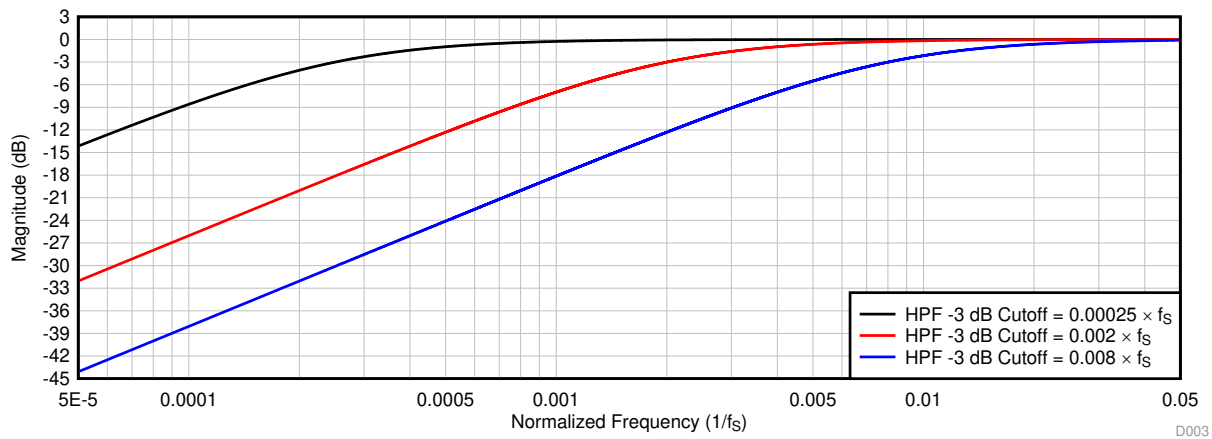
Figure 33. HPF Filter Frequency Response Plot
