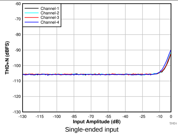
Figure 6. THD+N vs Input Amplitude
