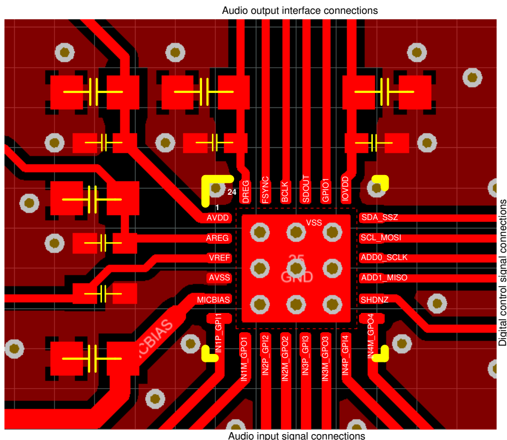
Figure 170. Layout Example
