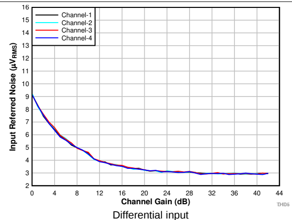
Figure 10. Input-Referred Noise vs Channel Gain
