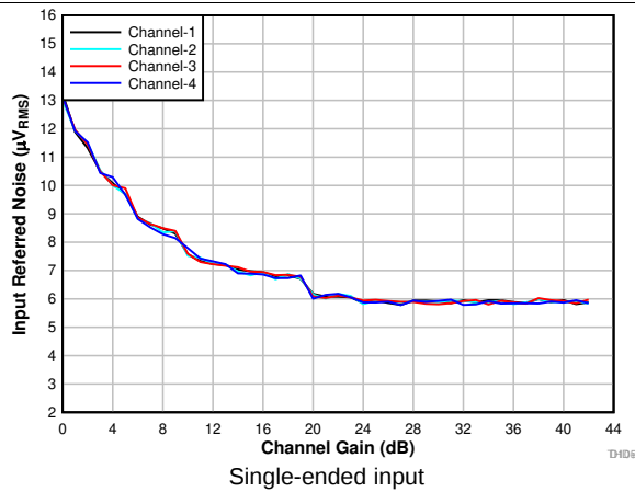
Figure 11. Input-Referred Noise vs Channel Gain
