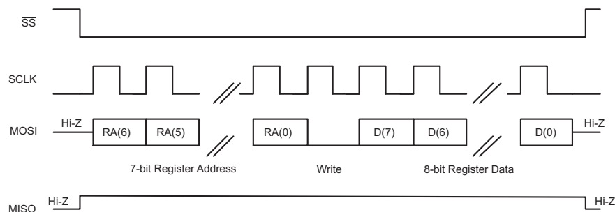
Figure 87. SPI Single-Byte Write Transfer
