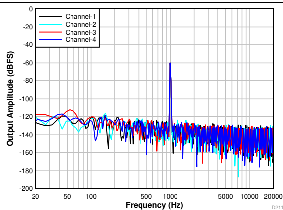
Figure 166. FFT With a -60-dBr Input
