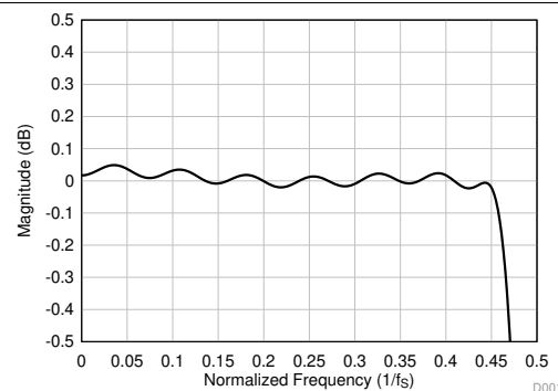
Figure 36. Linear Phase Decimation Filter Pass-Band Ripple
