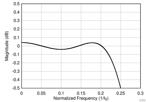
Figure 50. Linear Phase Decimation Filter Pass-Band Ripple
