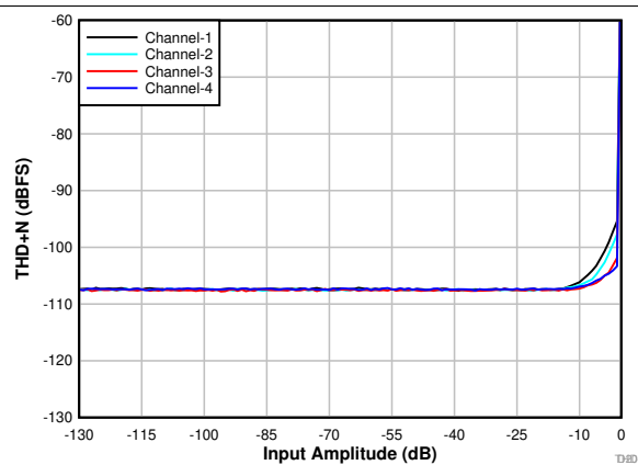
Figure 167. THD+N vs Input Amplitude
