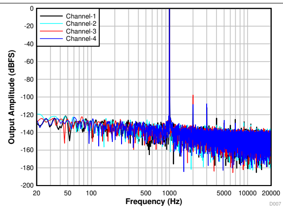
Figure 16. FFT With a -1-dBr Input
