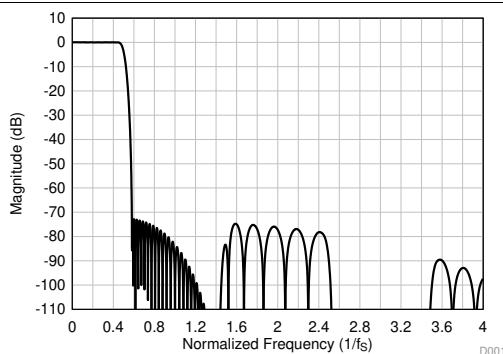
Figure 35. Linear Phase Decimation Filter Magnitude Response
