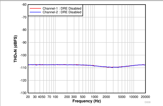
Figure 7-11. THD+N vs Input Frequency With a -60-dBr Input
