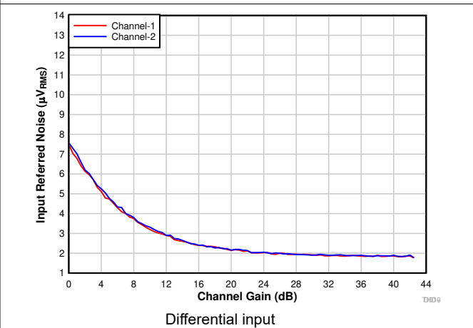
Figure 7-13. Input-Referred Noise vs Channel Gain
