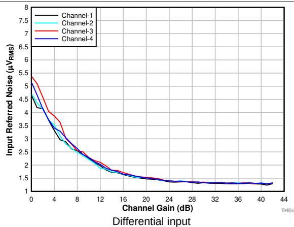
Figure 13. Input-Referred Noise vs Channel Gain
