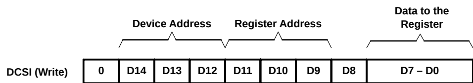
Figure 3-13. Direct Communication DCSI Data Format
