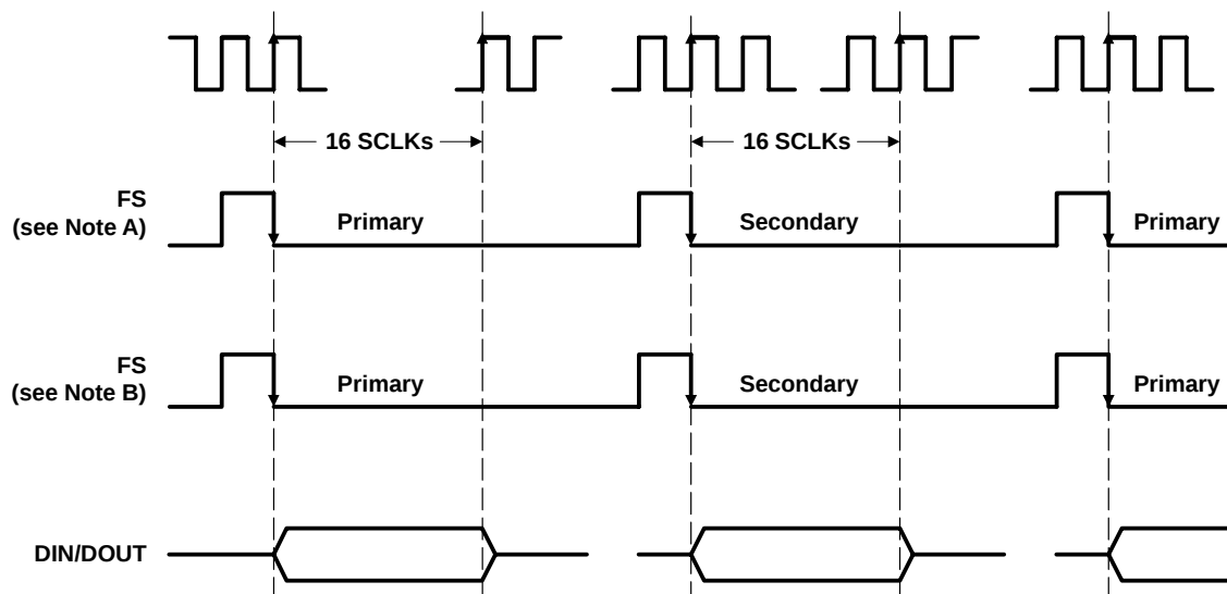
Figure 2–13. Master Device Frame-Sync Signal With Primary and Secondary Communication ( No Slaves)
