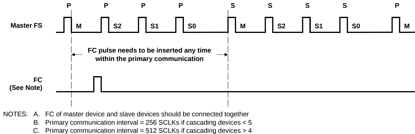
Figure 3–6. Output When Hardware Secondary Serial Communication Is Requested (Three Slaves)
