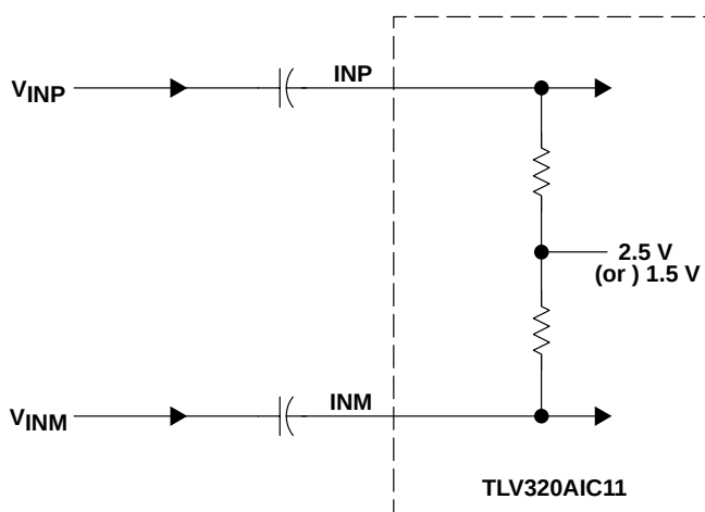
Figure 2–17. INP and INM Internal Self-Biased Circuit (2.5 V for 5-V Operation and 1.5 V for 3-V Operation)
