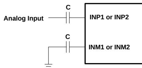
Figure 3–3. Single-Ended Input
