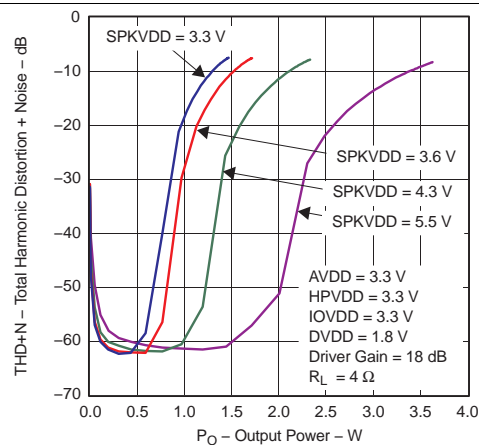
Figure 4-10. Total Harmonic Distortion + Noise vs Output Power Class-D Speaker-Driver Output Power ( R_L = 4 \Omega )
