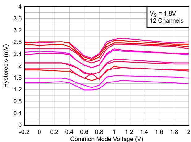
Figure 5-8. Hysteresis vs. Common-Mode, 1.8V
