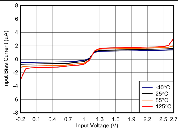
Figure 6-22. Bias Current vs. Input Voltage, 2.5 V
