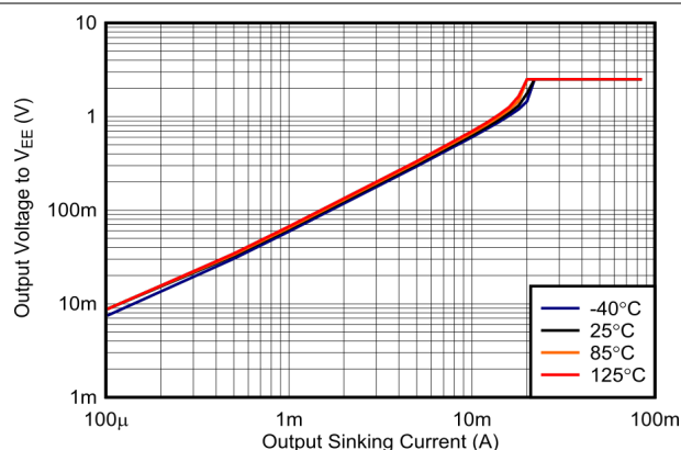
Figure 6-26. Output Voltage vs. Output Sinking Current, 2.5 V
