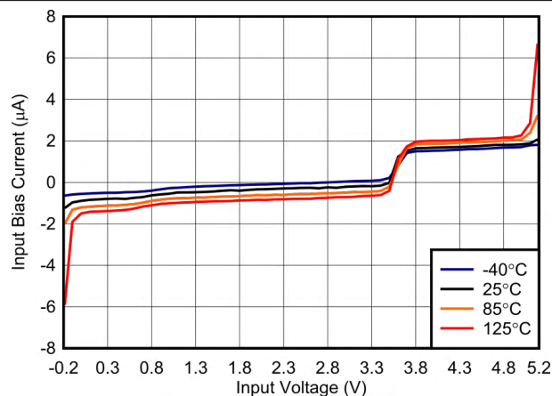
Figure 6-24. Bias Current vs. Input Voltage, 5 V
