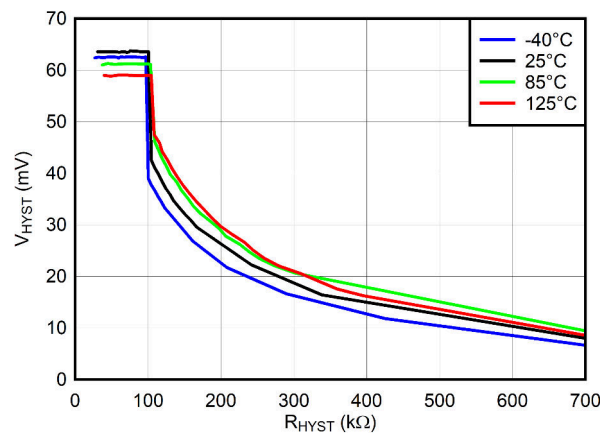
Figure 7-4. V HYST (mV) vs R HYST (kΩ), V CC = 3.3V
