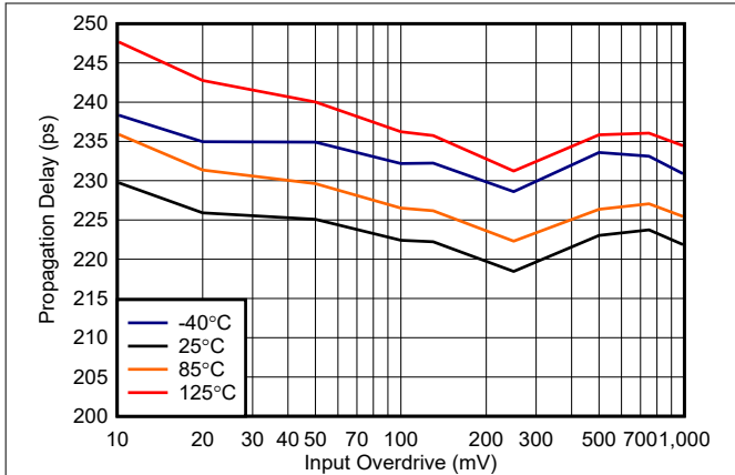
Figure 6-15. Propagation Delay vs. Overdrive, 3.3 V
