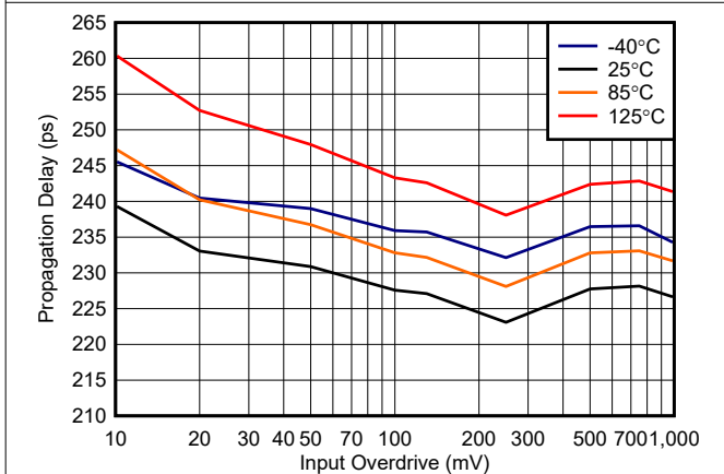
Figure 6-17. Propagation Delay vs. Overdrive, 5 V
