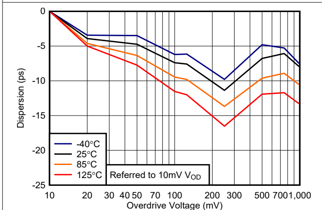
Figure 6-19. Dispersion vs. Overdrive, 3.3 V
