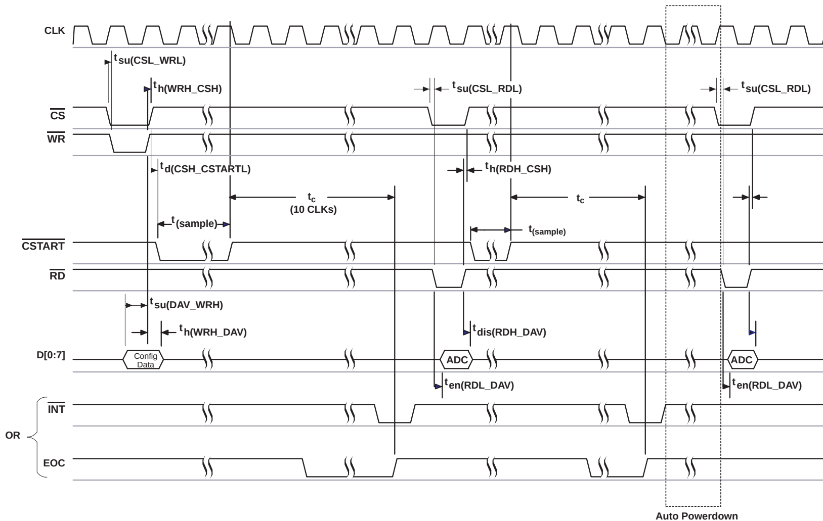
Figure 4. Input Conversion – Hardware \overline{CSTART} , External Clock
