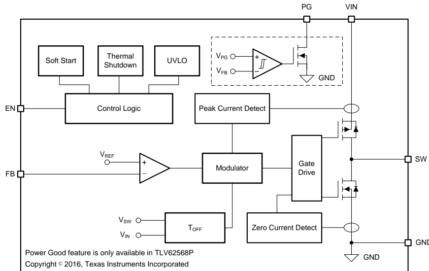
Figure 4. TLV62568 Functional Block Diagram
