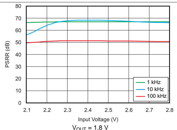
Figure 12. Power-Supply Ripple Rejection vs Input Voltage
