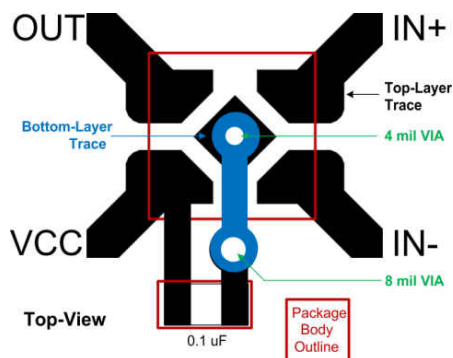
Figure 10-1. Layout Example
