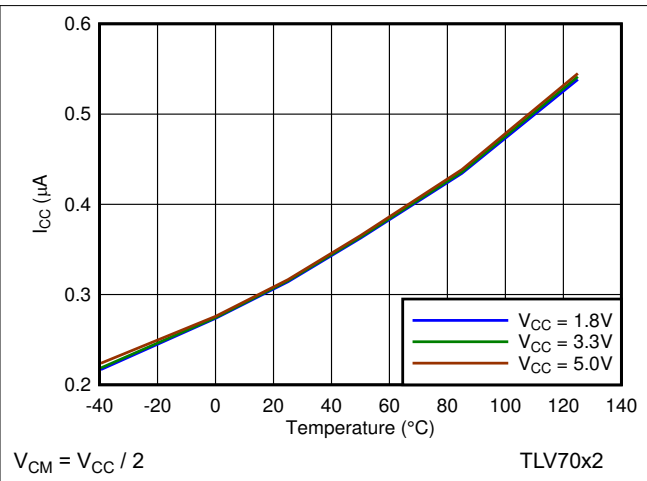
Figure 6-28. I_{CC} vs Temperature
