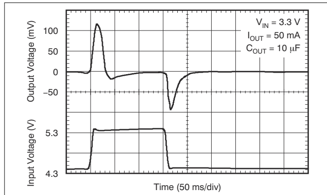
Figure 6-25. Line Transient Response for Legacy Chip
