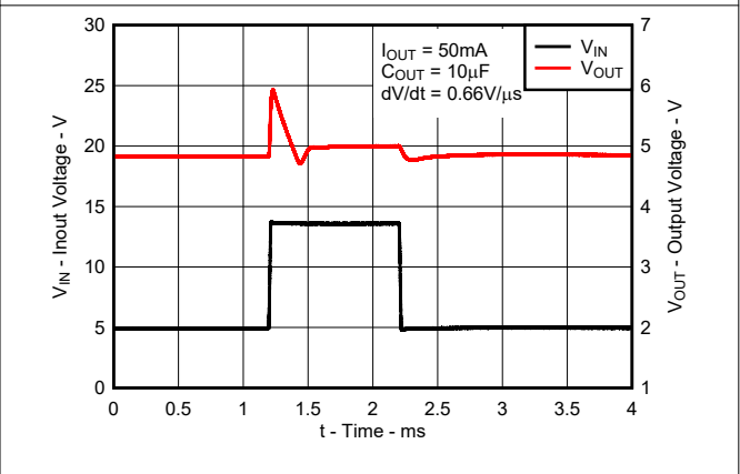
Figure 6-30. Dropout Exit Transient Response for New Chip
